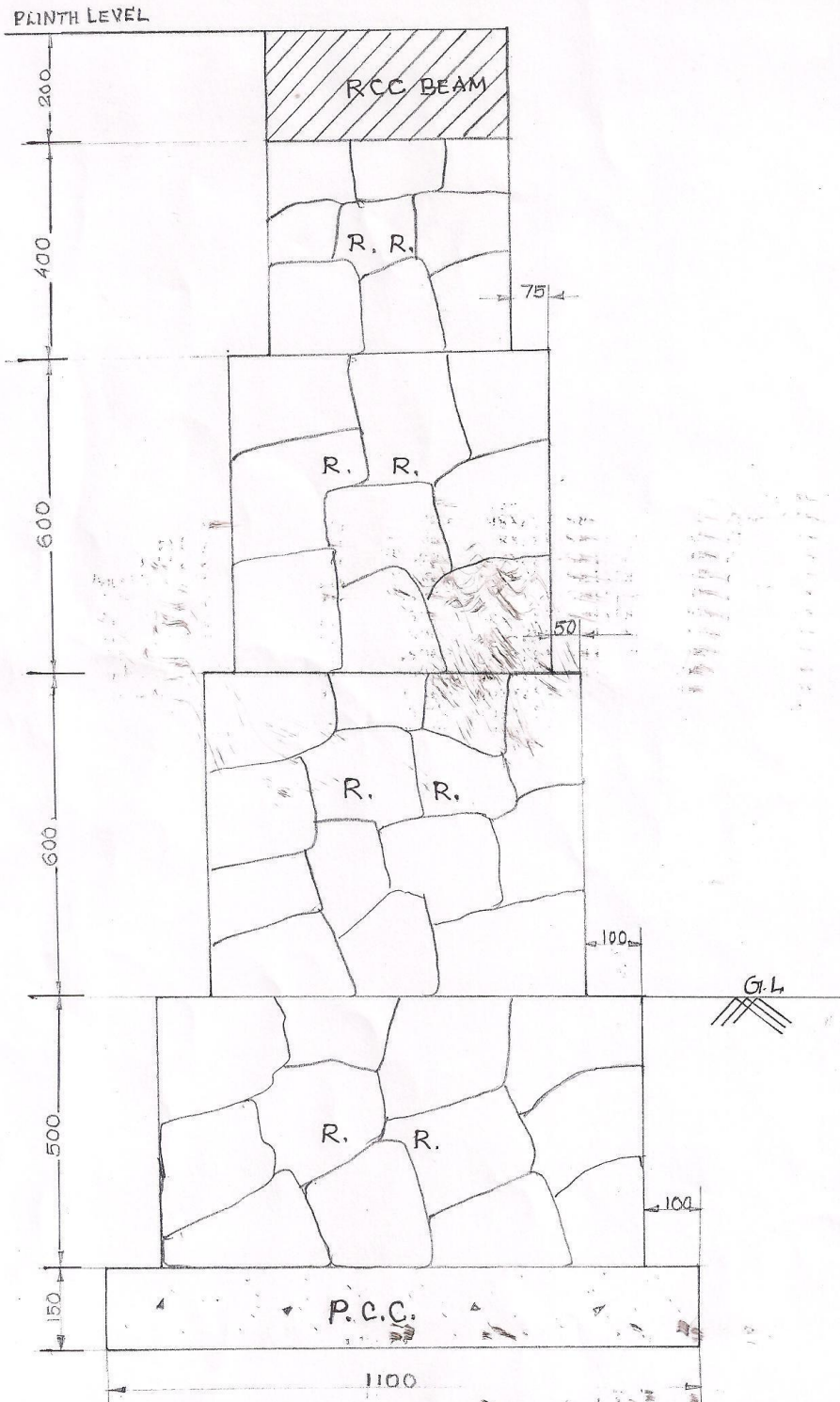
SECTION OF FOUNDATION FOR COMPOUND WALL FOR KOTTAPPURM TERMINAL SCALE- 1:100 ALL DIMENSIONS ARE IN mm
