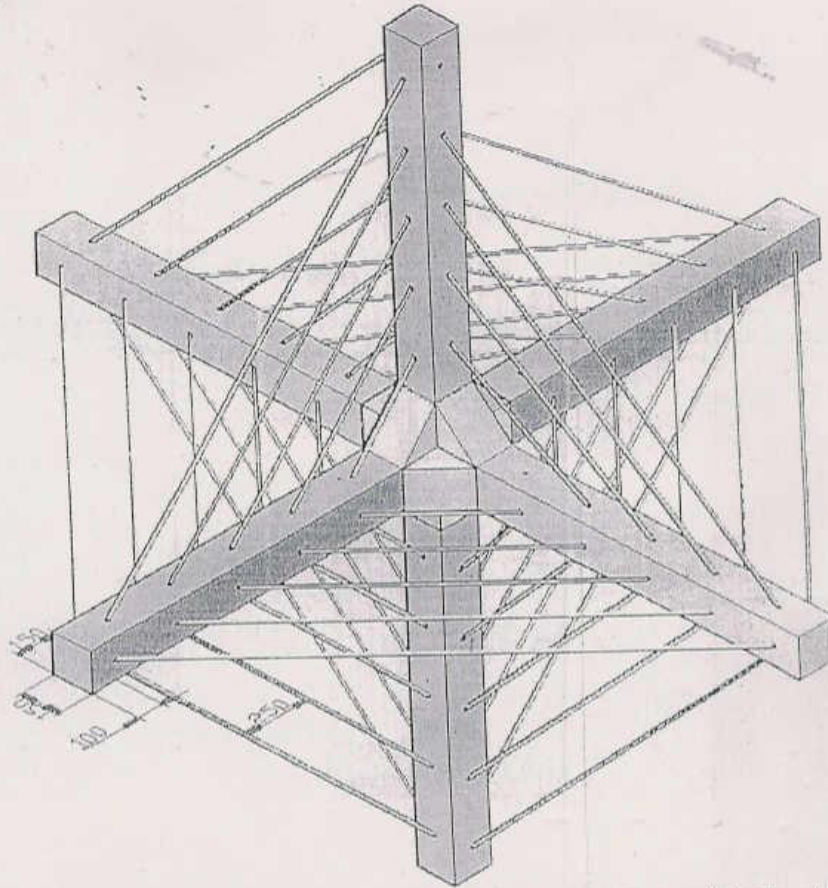
Drawing no. TYP-9: Typical Layout of RCC Kellner Jetty of 3m length and 15cm thickness with 15cm x 15cm haunch at junction mesh with 4mm GI Wire
