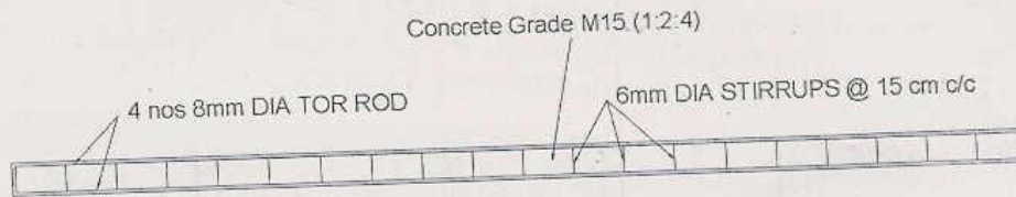
DETAILS OF LONGITUDINAL REINFORCEMENT IN RCC KELLNER JETTY
